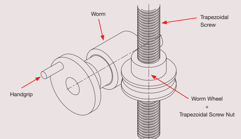
KWGDL Duplex Worm Wheels and AGDL Worm Wheels used for indexing and driving, for accurate filling of a fixed amount of ingredients
